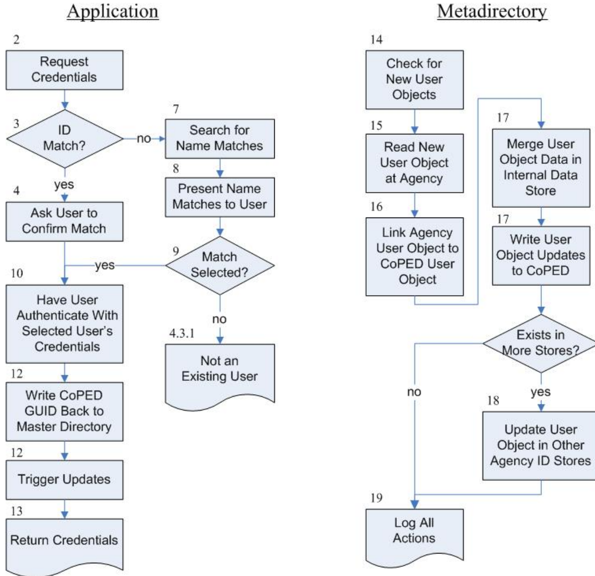
Figure 3 – Existing Identity Scenario Flow
