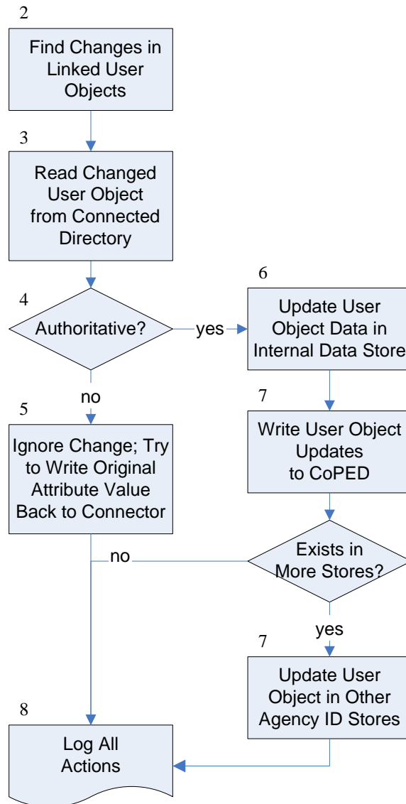
Figure 4 – User Attribute Change Scenario Flow
