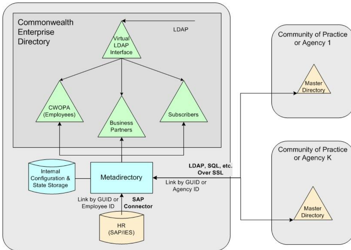
Figure 1 – Identity Data Synchronization Architecture
