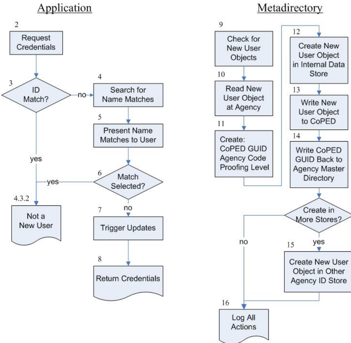
New Identity Scenario Flow
